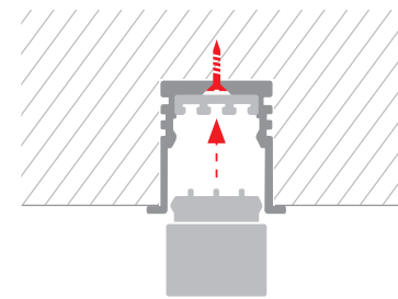
Colocar luminaria
